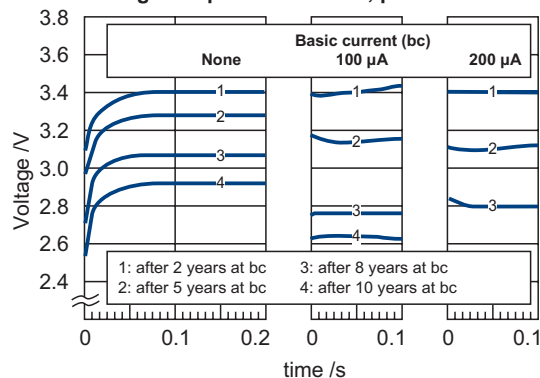
Voltage Response at +25 °C, pulse: 120 mA
